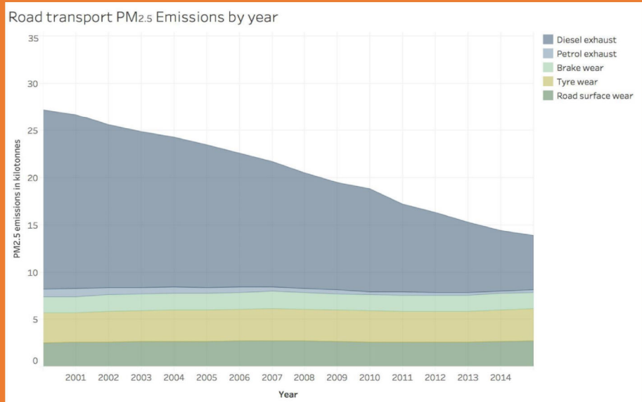
Figure 1. PM 2.5 emissions from road transport, 2000-2015. Source: NAEI 2015
