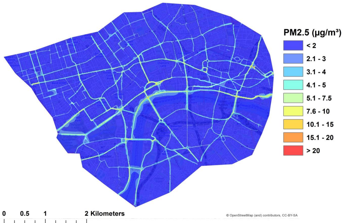
Figure 16: Modelled non-exhaust PM 2.5 annual average concentration for 2016 within the London Congestion Charging Zone.
